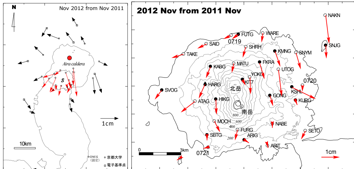
Fig. 5 Vectors of horizontal displacement around the Aira caldera (left) and at Sakurajima (right). Horizontal displacement vectors are shown by arrows, relative to Station ONEG. Central cones of Sakurajima are indicated by “S” in the left figure. The dot indicates pressure source of Mogi type.
