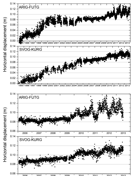
Fig. 3 Daily horizontal displacements along north-east baseline between ARIG and FUTG and east-west baseline between SVOG and KURG. Lower figure is enlargement after 2006.
