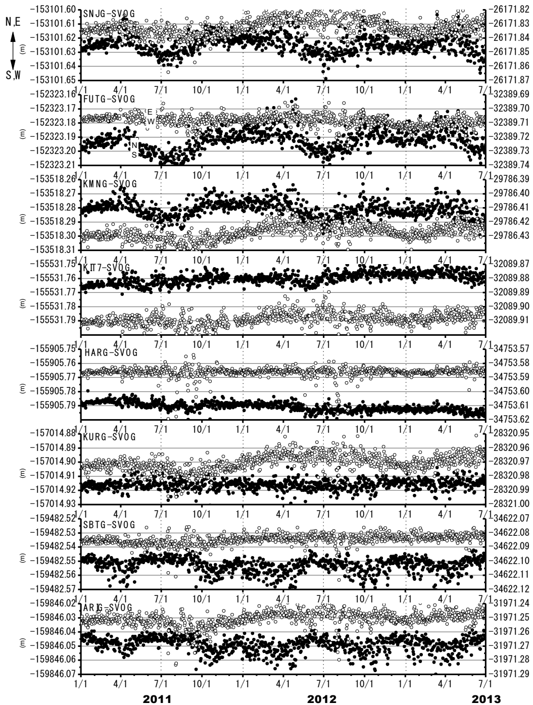
Fig. 4 Temporal change of location of GPS stations referred station SVOG. Dots and open circles represent north-south and east-west components, respectively, in local Cartesian coordinate system. Origin of the Cartesian coordinate is located at 33°N and 131°E.
