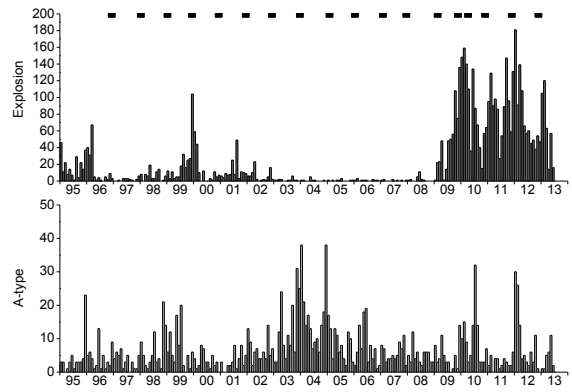
Fig. 2 Campaign periods of GPS measurement and activity of the Sakurajima volcano. Campaign periods are shown by bars at the top. Activity of the volcano is indicated by monthly numbers of explosion and A-type earthquake. Most of explosive eruptions occurred at the Showa crater after 2008. Numbers until June 2013 are plotted.
