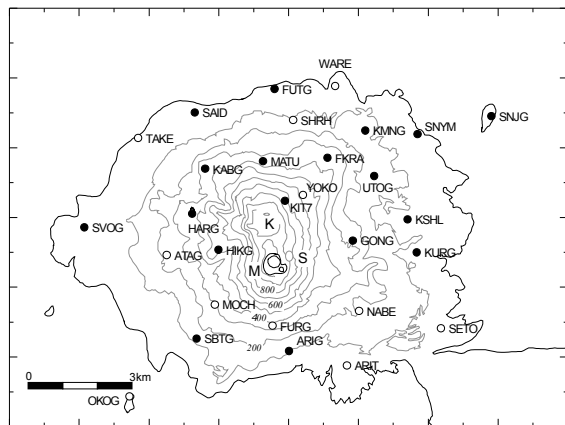
Fig. 1 Location of GPS stations and benchmarks. Dots and open circles indicate continuous GPS stations and benchmarks for campaigns, respectively. Top: GPS network around Aira caldera. Bottom: Sakurajima network.
